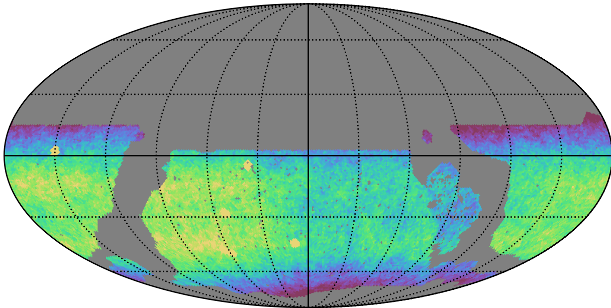
noroll_v3.4_10yrs WFD z band: CoaddM5
