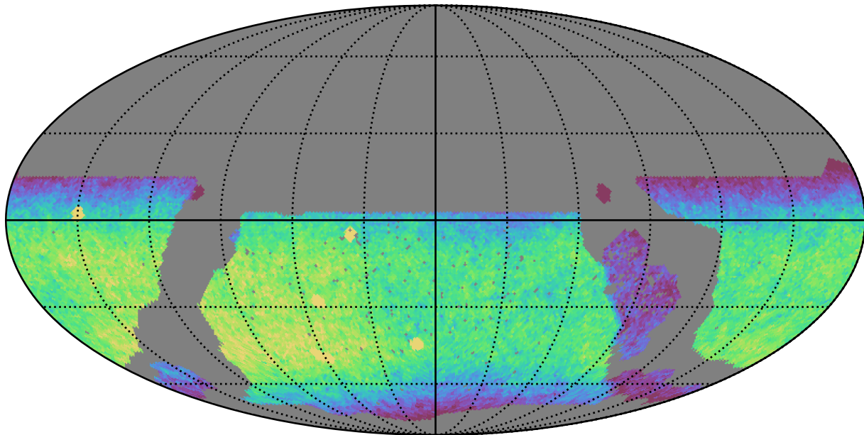
noroll_v3.4_10yrs WFD y band: CoaddM5
