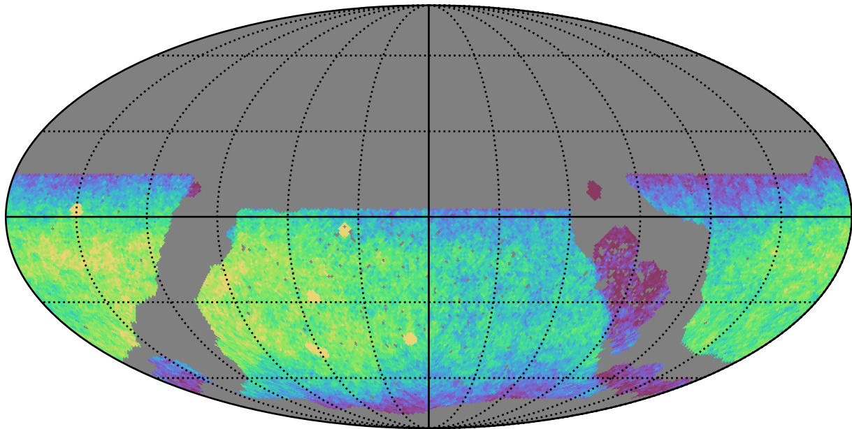
noroll_v3.4_10yrs WFD u band: CoaddM5
