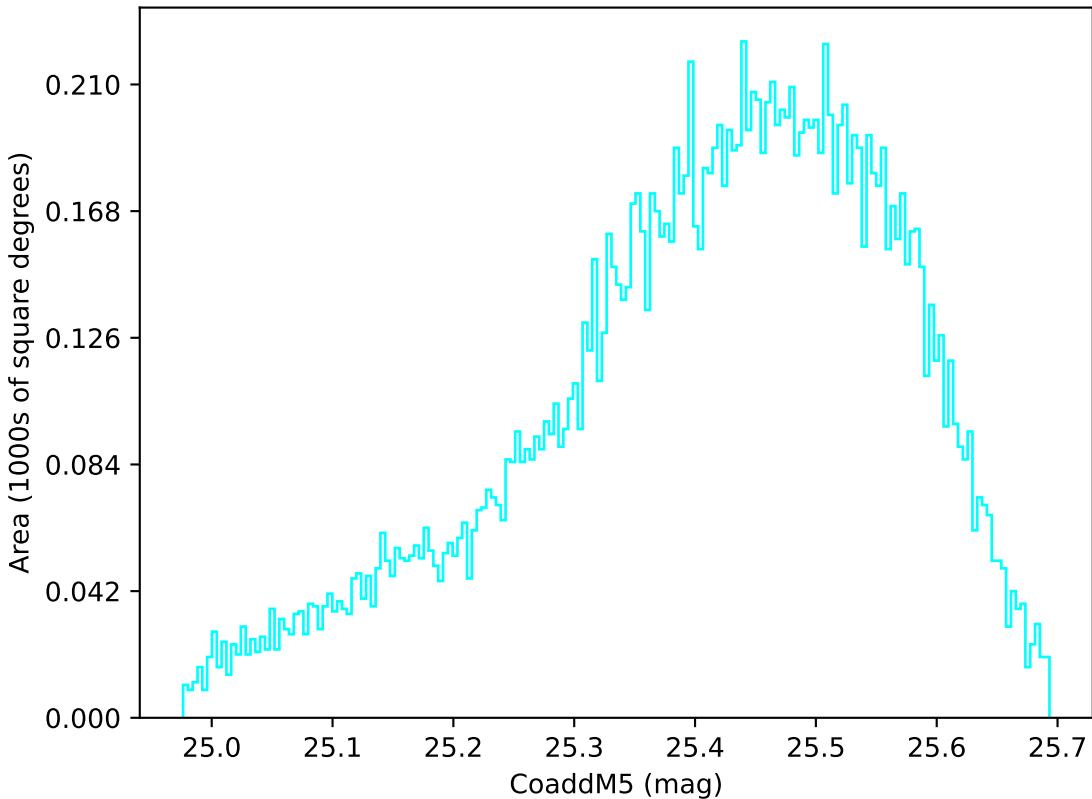
noroll_v3.4_10yrs WFD u band: CoaddM5
