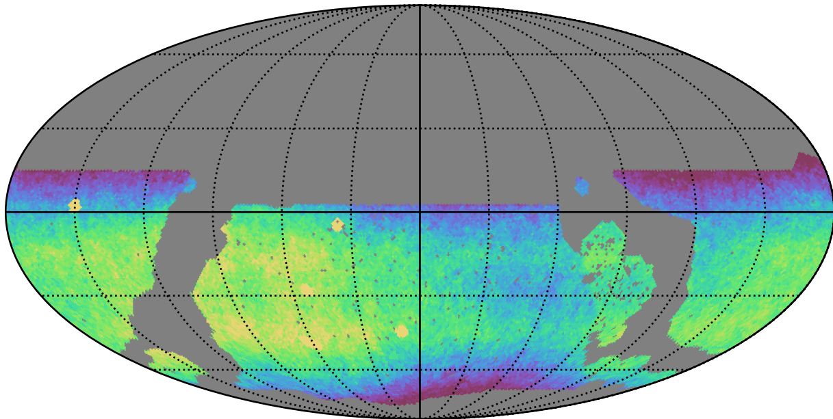
noroll_v3.4_10yrs WFD r band: CoaddM5
