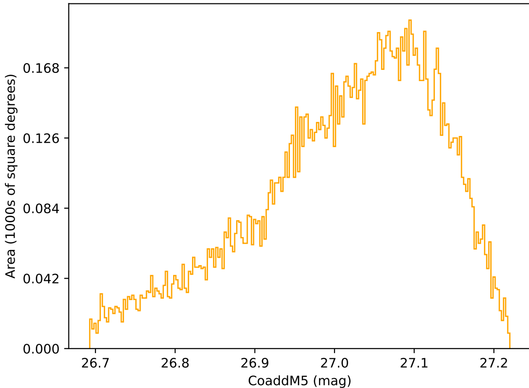
noroll_v3.4_10yrs WFD r band: CoaddM5
