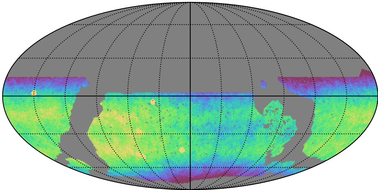
noroll_v3.4_10yrs WFD i band: CoaddM5
