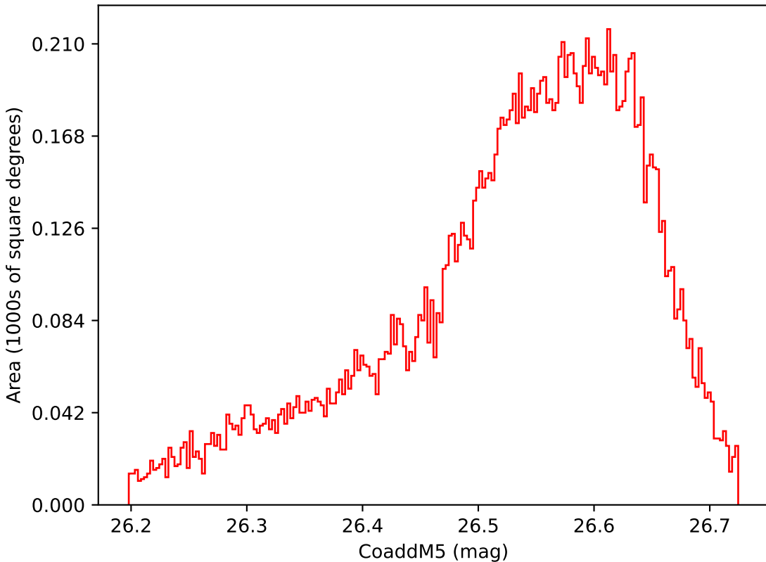
noroll_v3.4_10yrs WFD i band: CoaddM5
