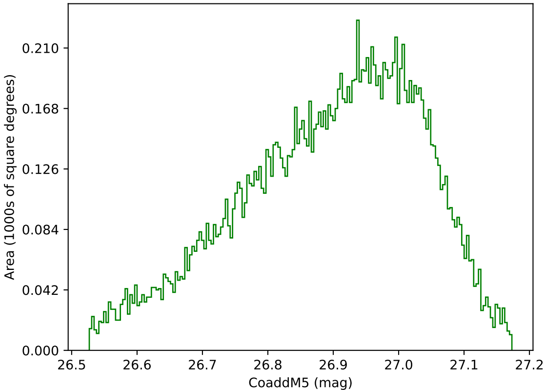
noroll_v3.4_10yrs WFD g band: CoaddM5
