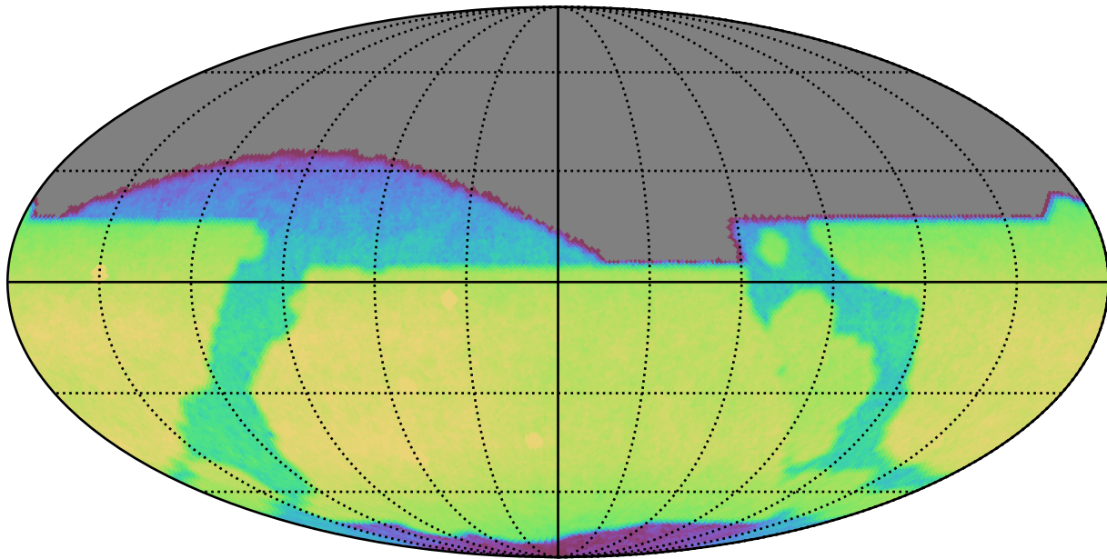
noroll_v3.4_10yrs All sky z band: CoaddM5
