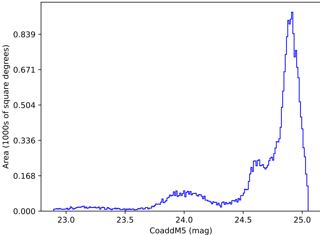
noroll_v3.4_10yrs All sky y band: CoaddM5
