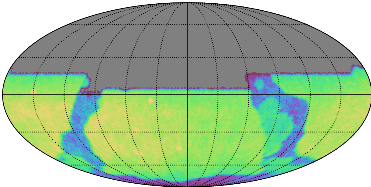
noroll_v3.4_10yrs All sky u band: CoaddM5
