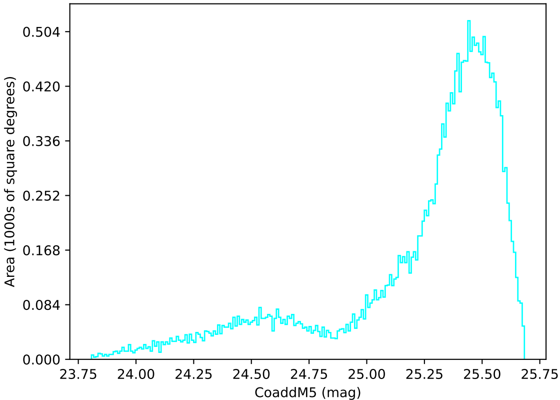
noroll_v3.4_10yrs All sky u band: CoaddM5
