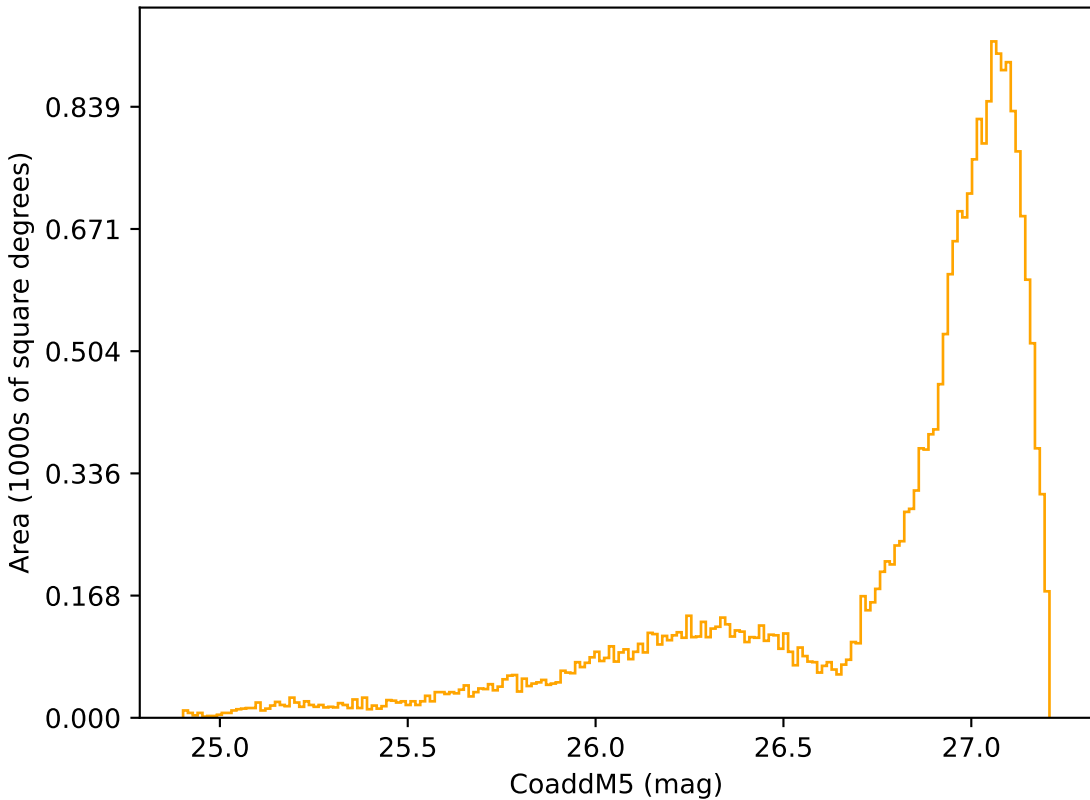
noroll_v3.4_10yrs All sky r band: CoaddM5
