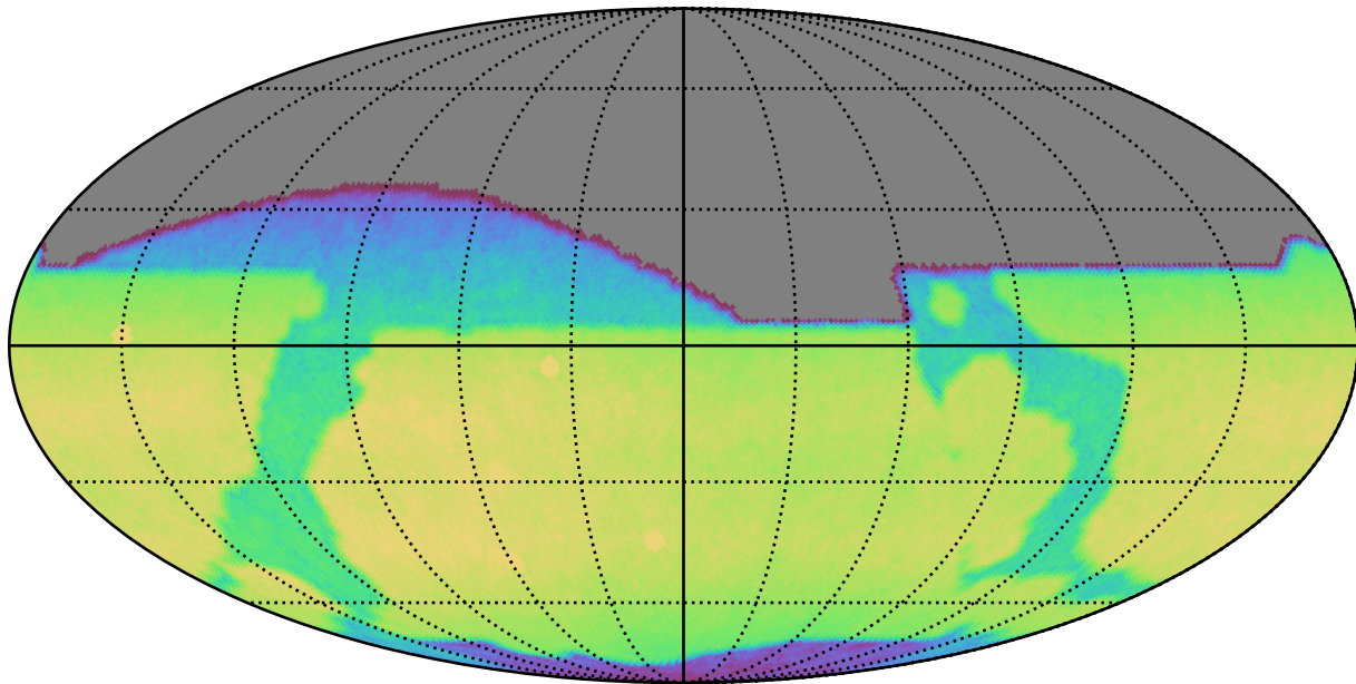
noroll_v3.4_10yrs All sky i band: CoaddM5
