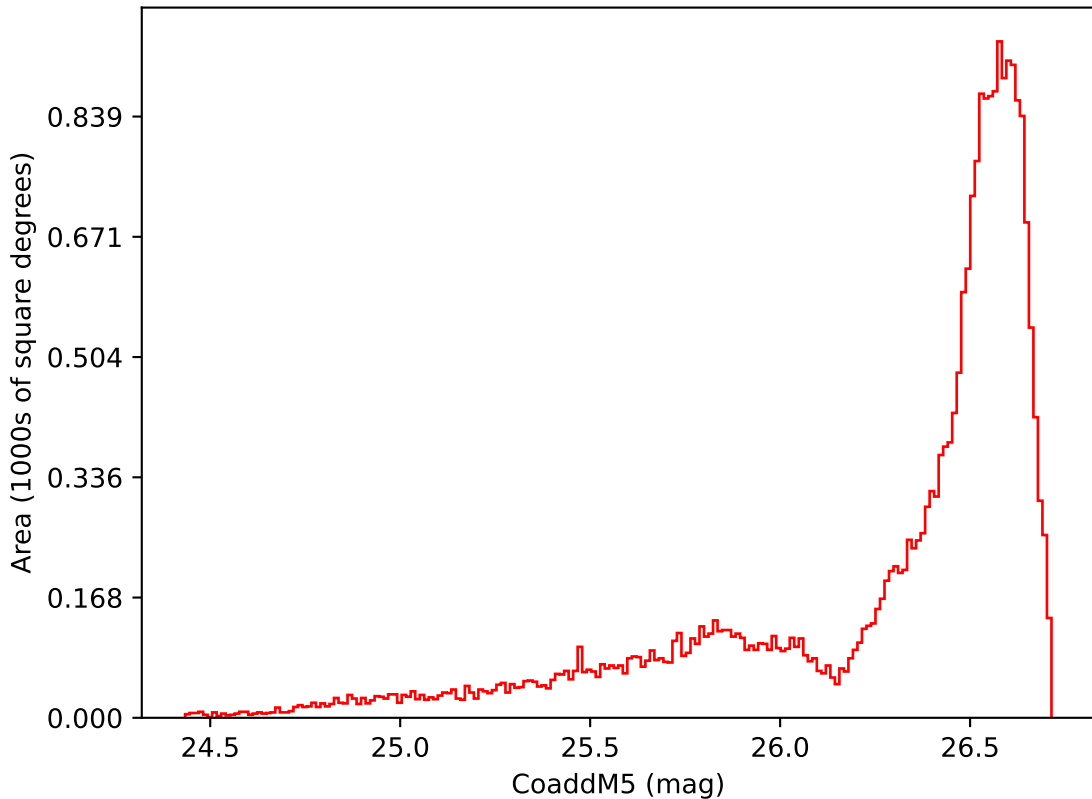
noroll_v3.4_10yrs All sky i band: CoaddM5
