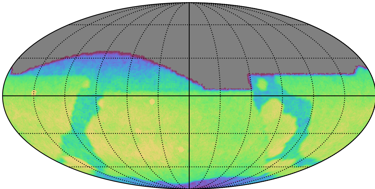
noroll_v3.4_10yrs All sky g band: CoaddM5
