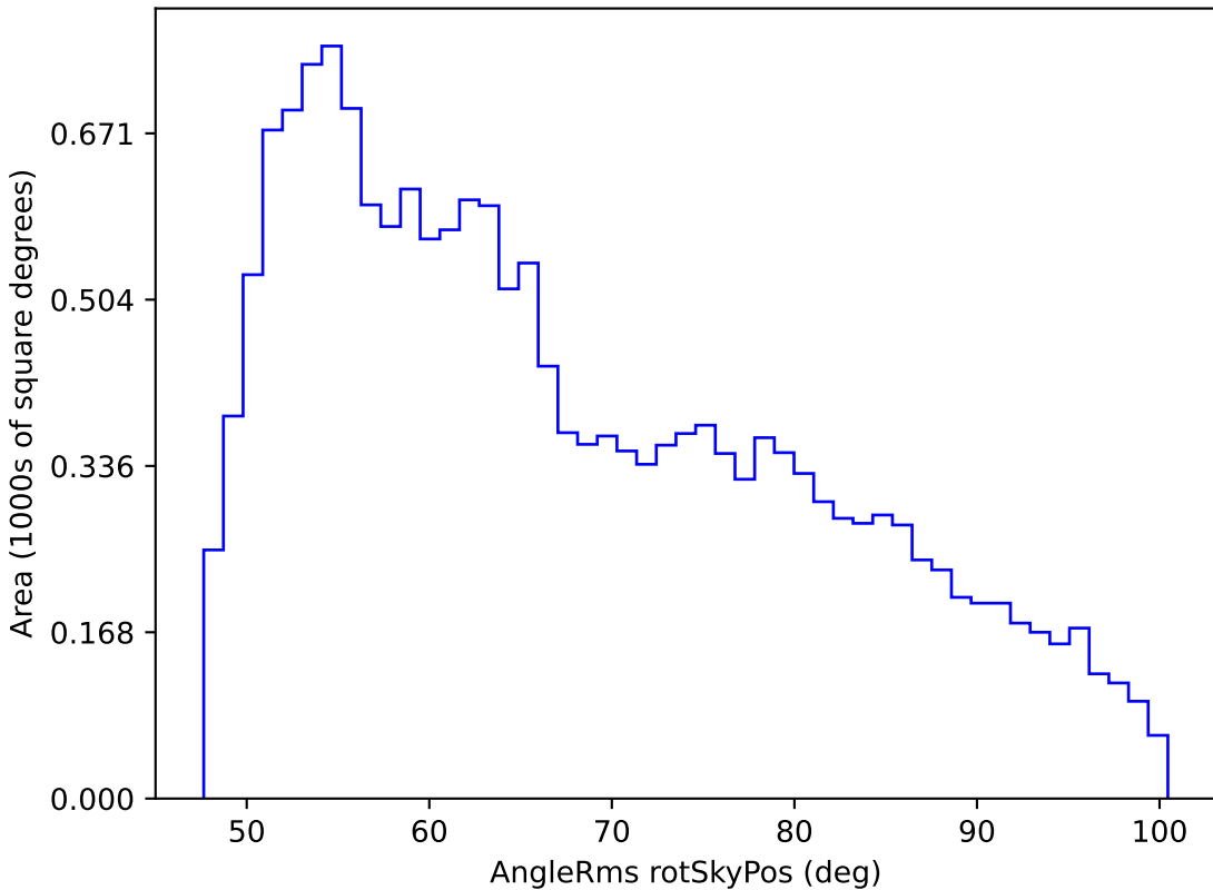
noroll_v3.4_10yrs WFD z band: AngleRms rotSkyPos
