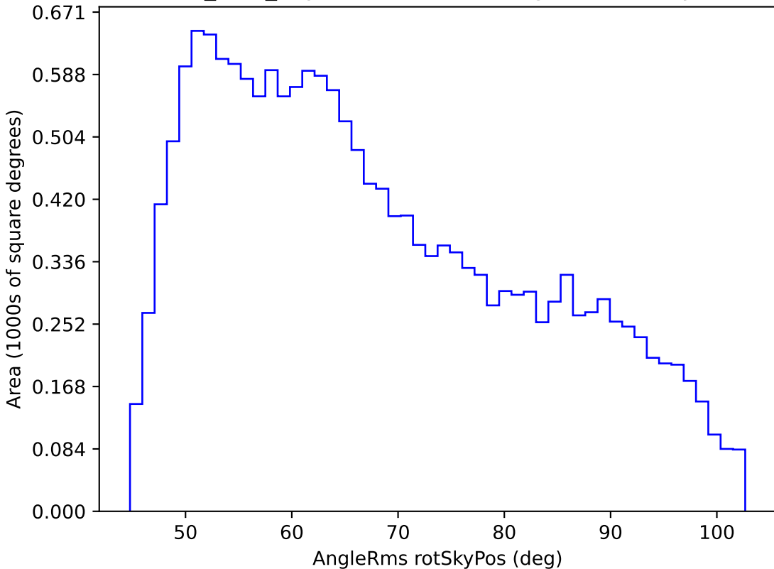
noroll_v3.4_10yrs WFD u band: AngleRms rotSkyPos
