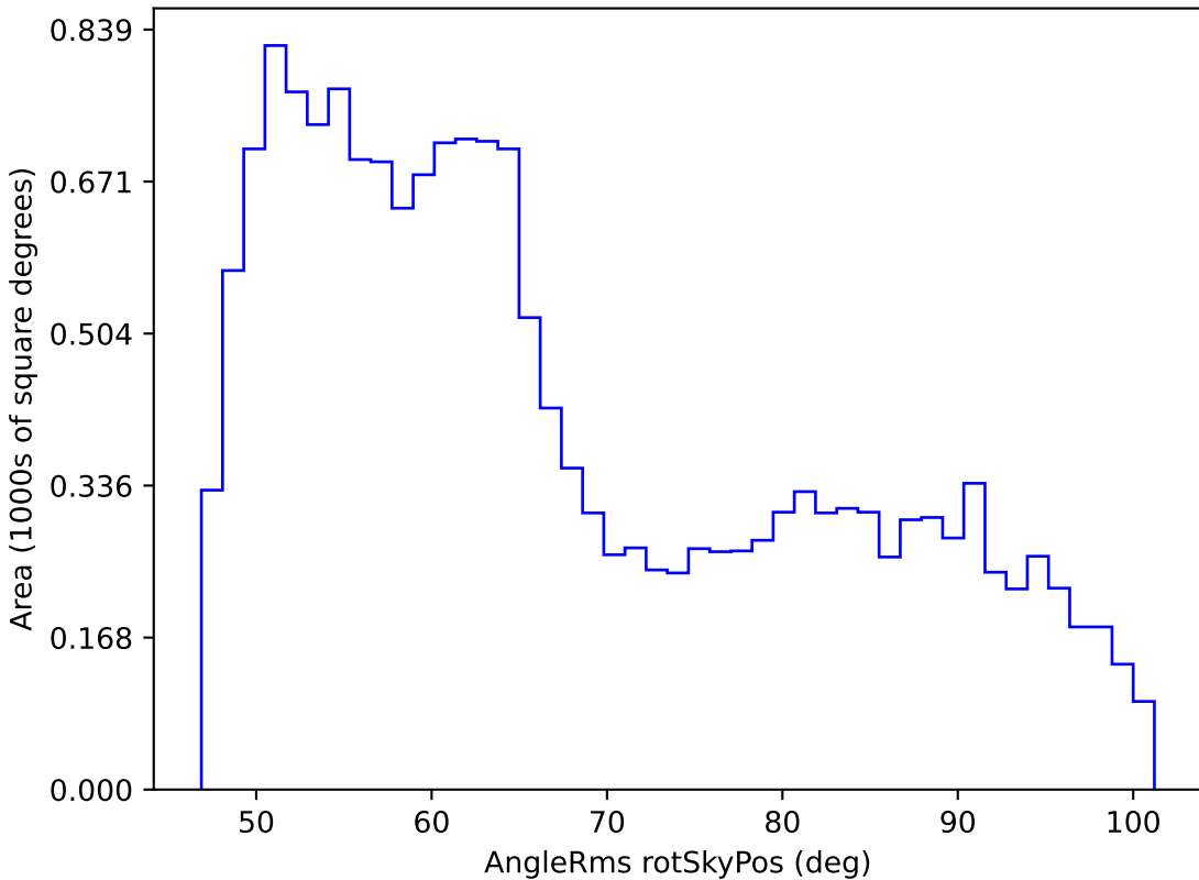
noroll_v3.4_10yrs WFD r band: AngleRms rotSkyPos
