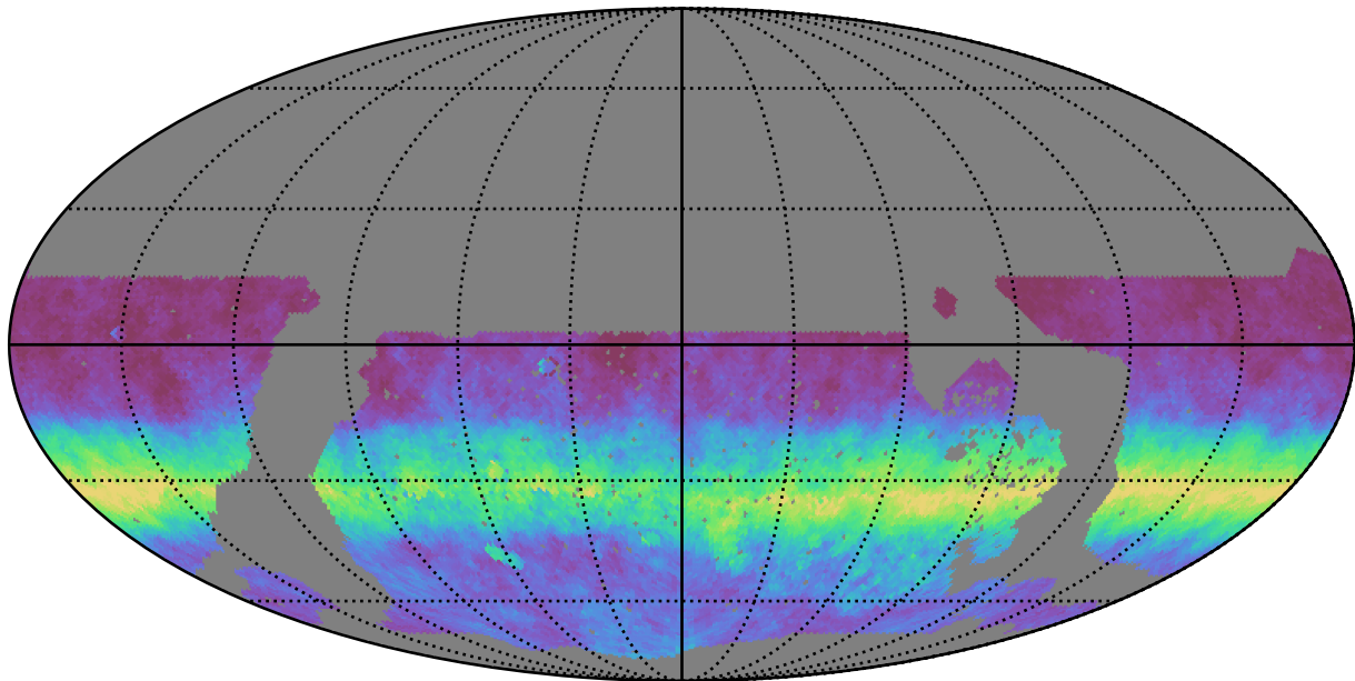
noroll_v3.4_10yrs WFD i band: AngleRms rotSkyPos
