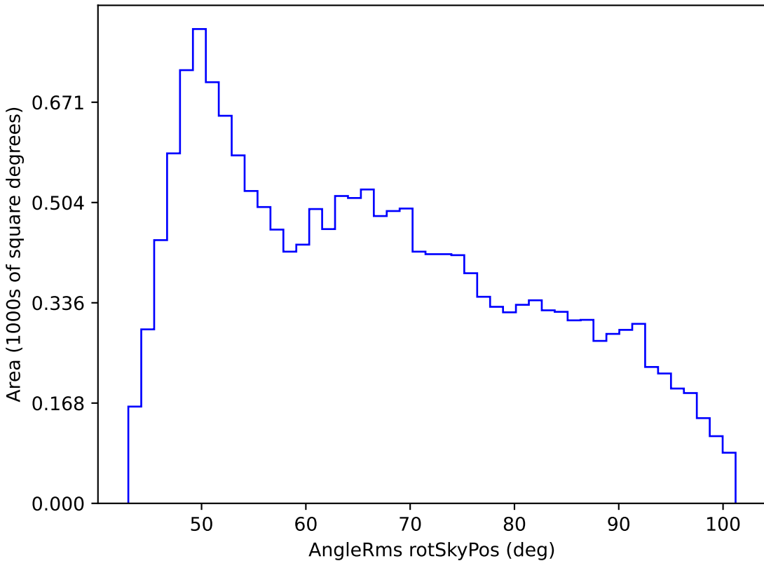
noroll_v3.4_10yrs WFD g band: AngleRms rotSkyPos
