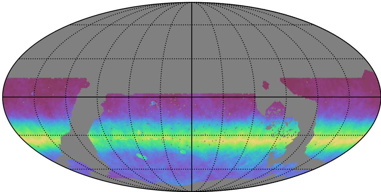
noroll_v3.4_10yrs WFD all bands: AngleRms rotSkyPos
