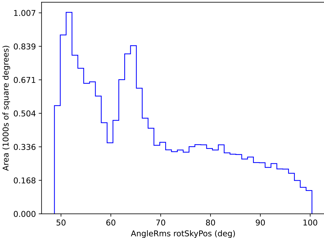
noroll_v3.4_10yrs WFD all bands: AngleRms rotSkyPos
