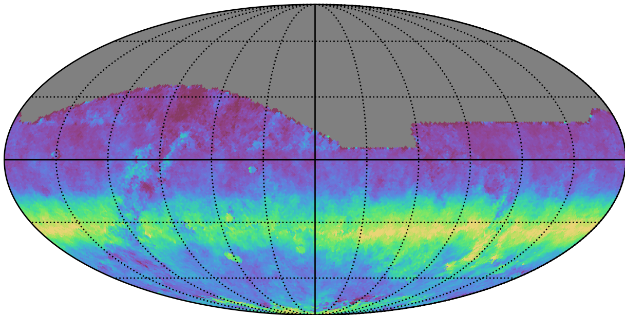
noroll_v3.4_10yrs All sky z band: AngleRms rotSkyPos
