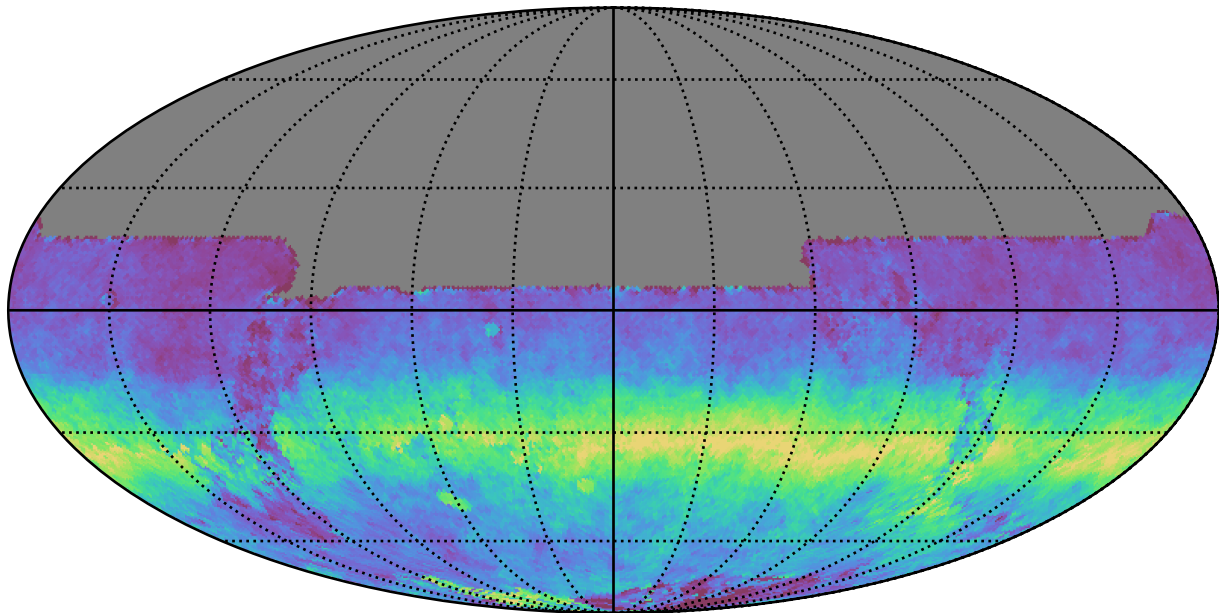
noroll_v3.4_10yrs All sky y band: AngleRms rotSkyPos
