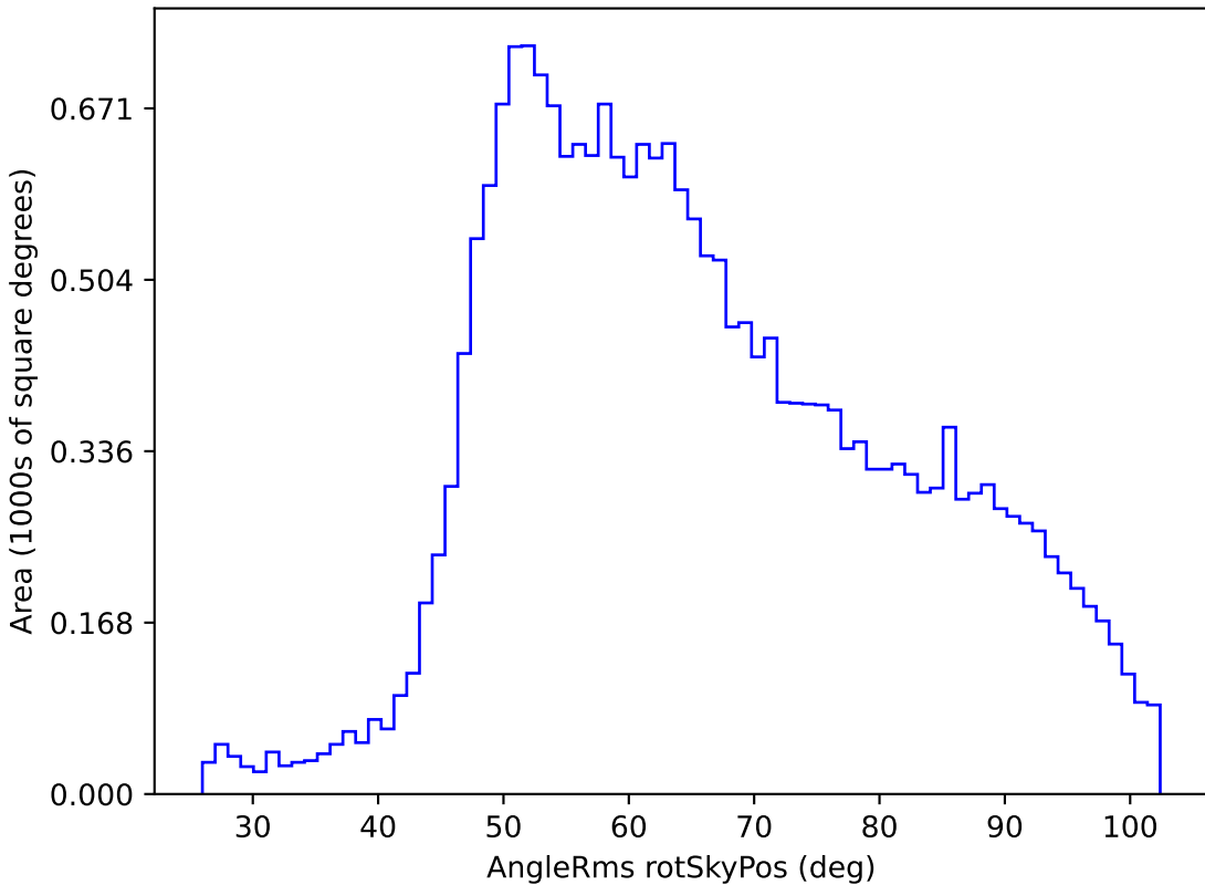
noroll_v3.4_10yrs All sky u band: AngleRms rotSkyPos
