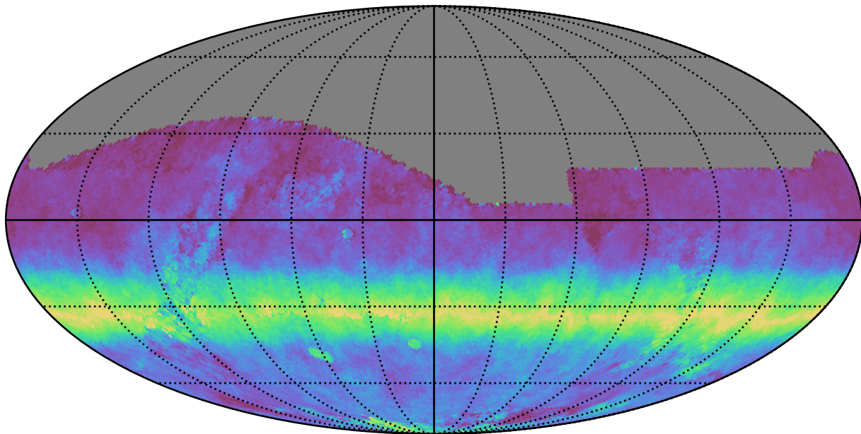
noroll_v3.4_10yrs All sky r band: AngleRms rotSkyPos
