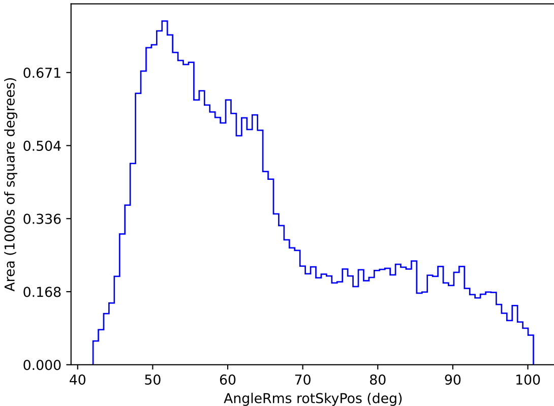
noroll_v3.4_10yrs All sky r band: AngleRms rotSkyPos
