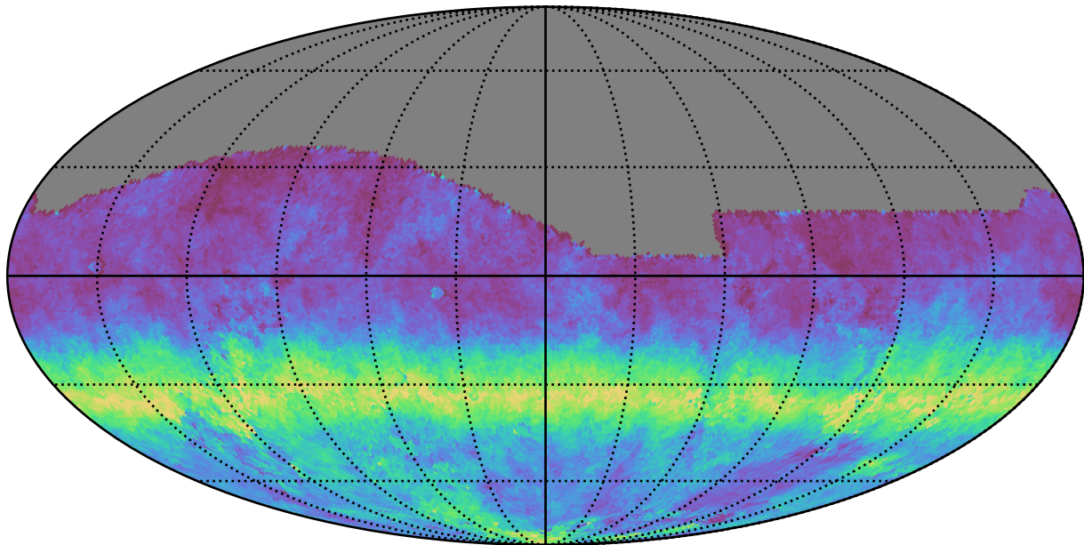
noroll_v3.4_10yrs All sky g band: AngleRms rotSkyPos
