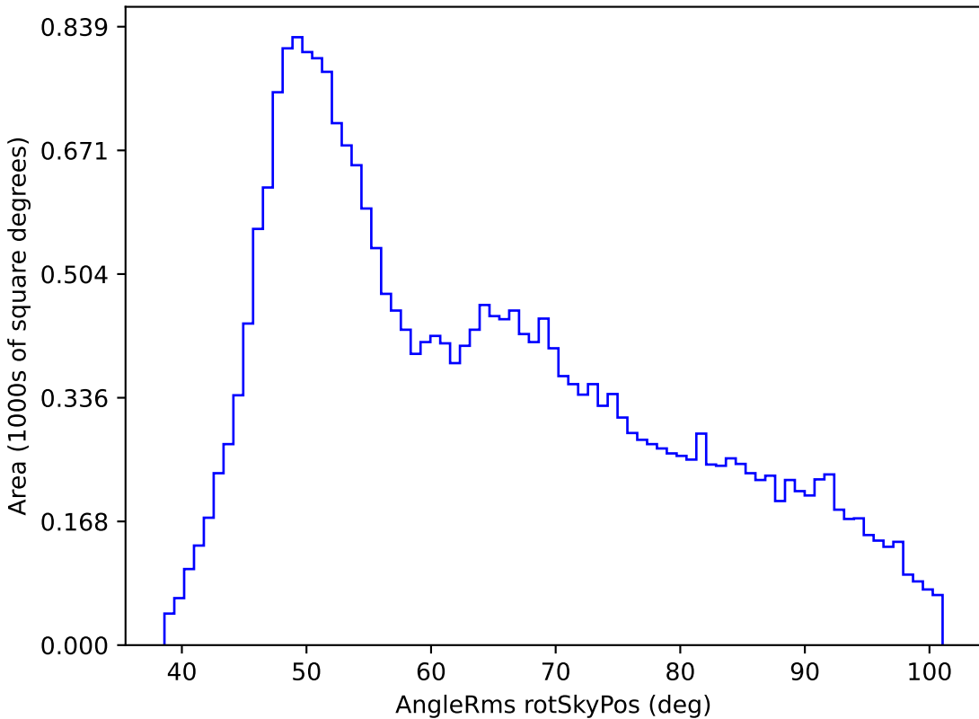
noroll_v3.4_10yrs All sky g band: AngleRms rotSkyPos
