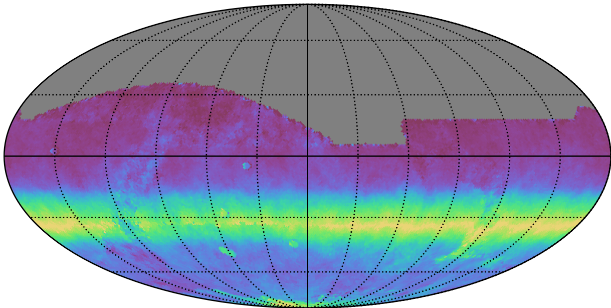
noroll_v3.4_10yrs All sky all bands: AngleRms rotSkyPos
