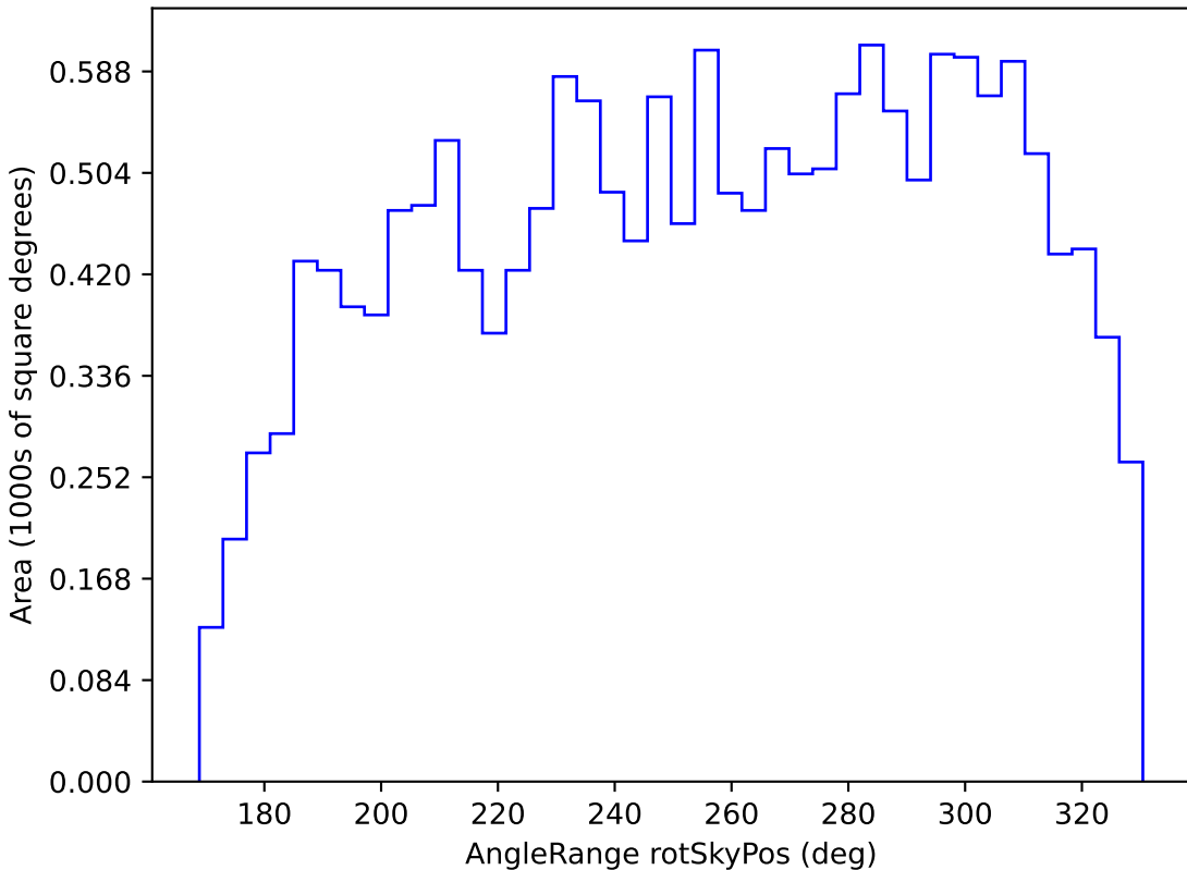
noroll_v3.4_10yrs WFD u band: AngleRange rotSkyPos
