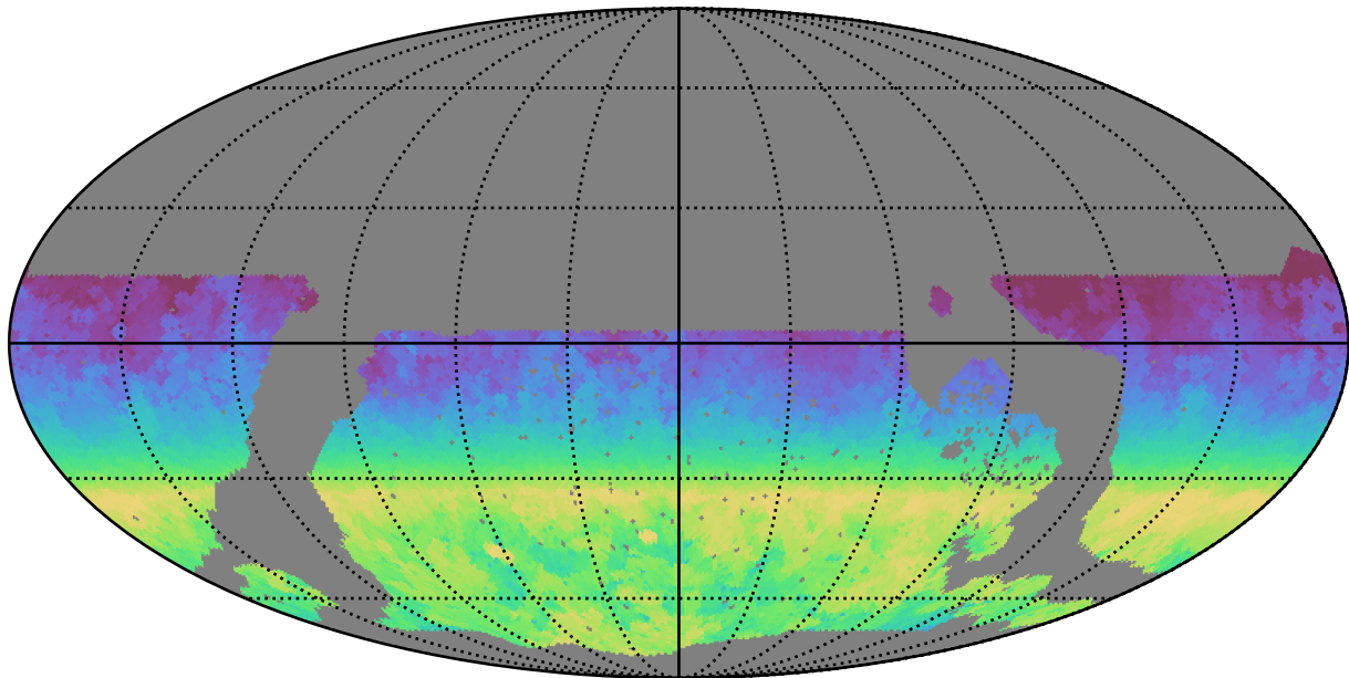
noroll_v3.4_10yrs WFD all bands: AngleRange rotSkyPos
