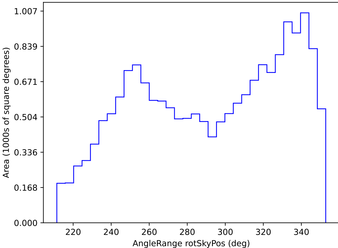
noroll_v3.4_10yrs WFD all bands: AngleRange rotSkyPos
