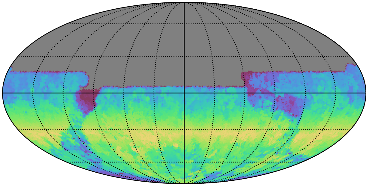
noroll_v3.4_10yrs All sky u band: AngleRange rotSkyPos
