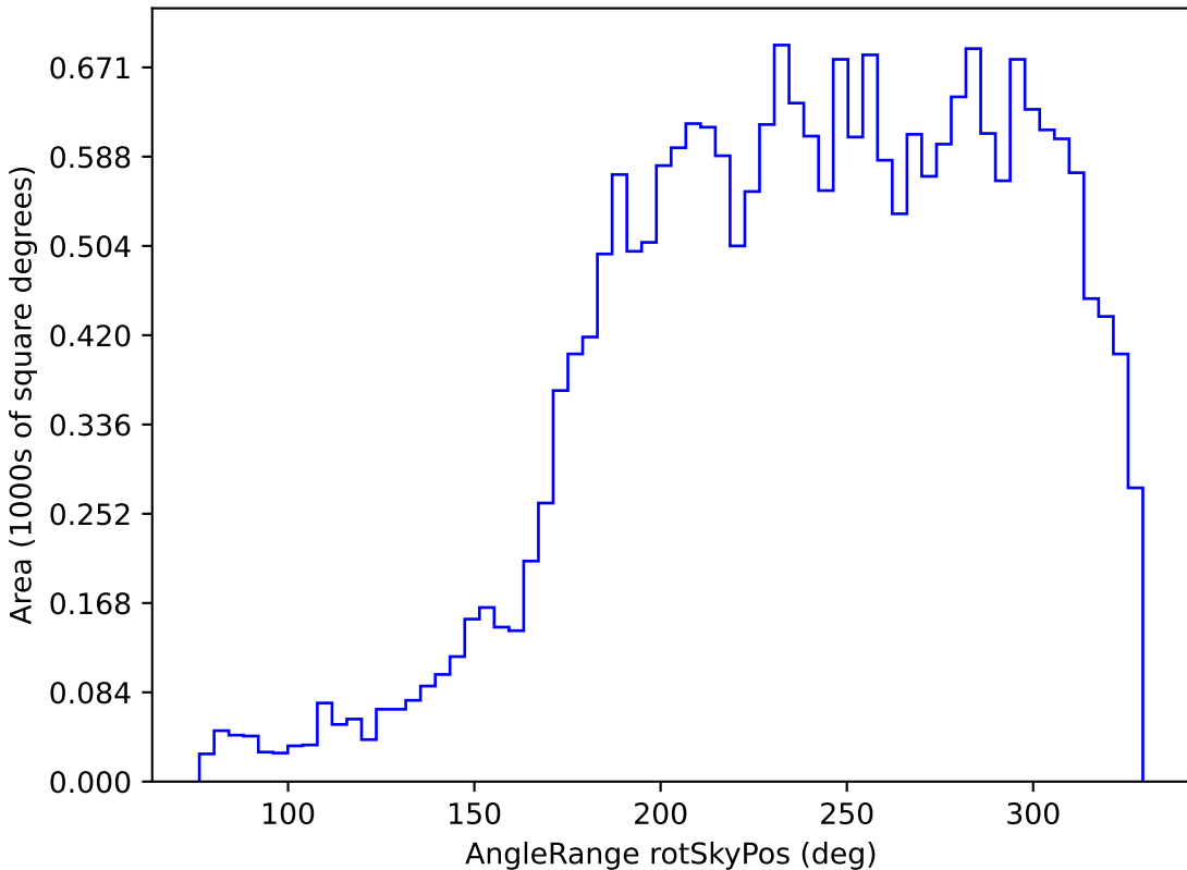
noroll_v3.4_10yrs All sky u band: AngleRange rotSkyPos
