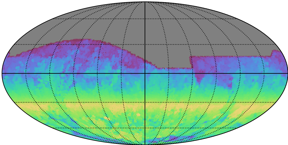
noroll_v3.4_10yrs All sky r band: AngleRange rotSkyPos
