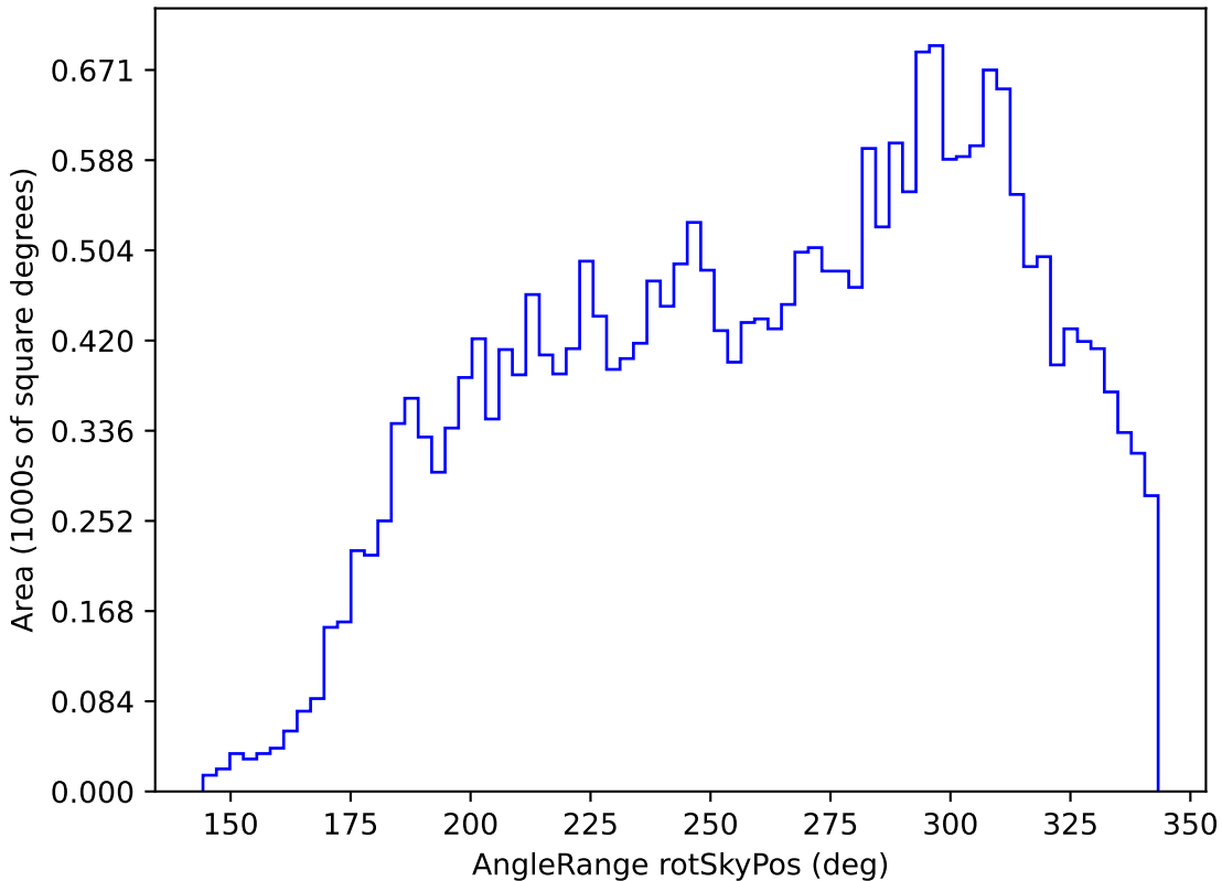
noroll_v3.4_10yrs All sky r band: AngleRange rotSkyPos
