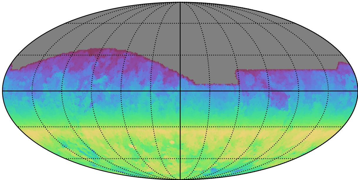
noroll_v3.4_10yrs All sky all bands: AngleRange rotSkyPos
