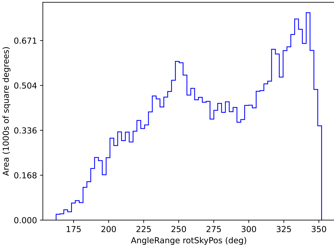
noroll_v3.4_10yrs All sky all bands: AngleRange rotSkyPos
