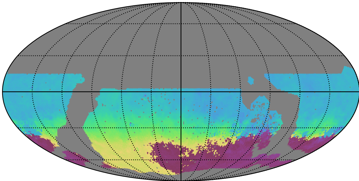
noroll_v3.4_10yrs WFD z band: AngleMean rotSkyPos
