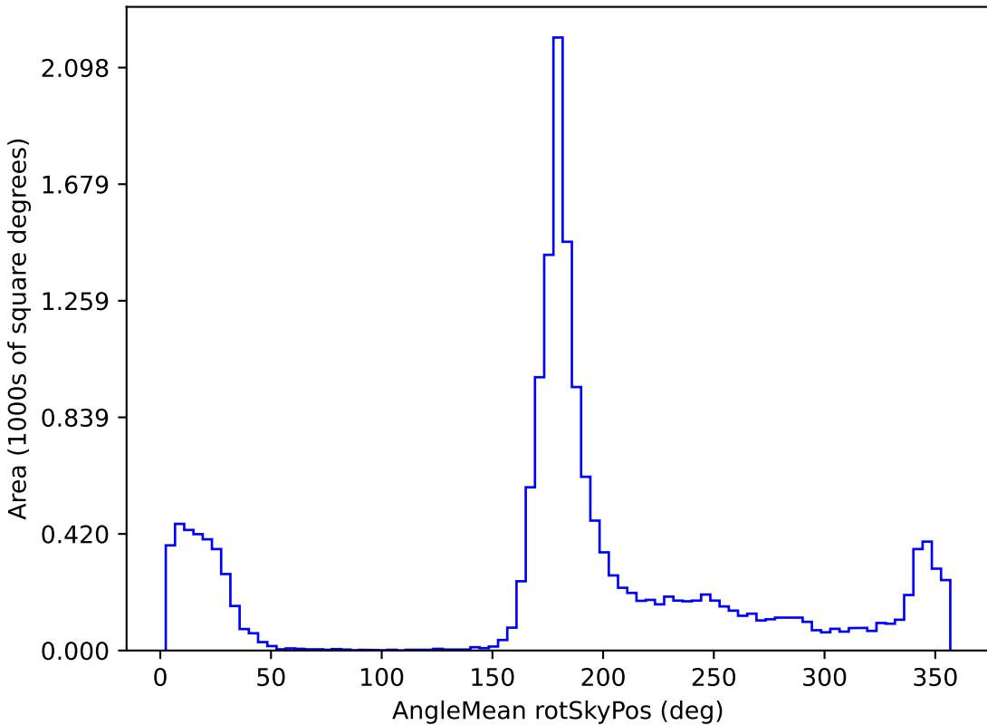
noroll_v3.4_10yrs WFD z band: AngleMean rotSkyPos
