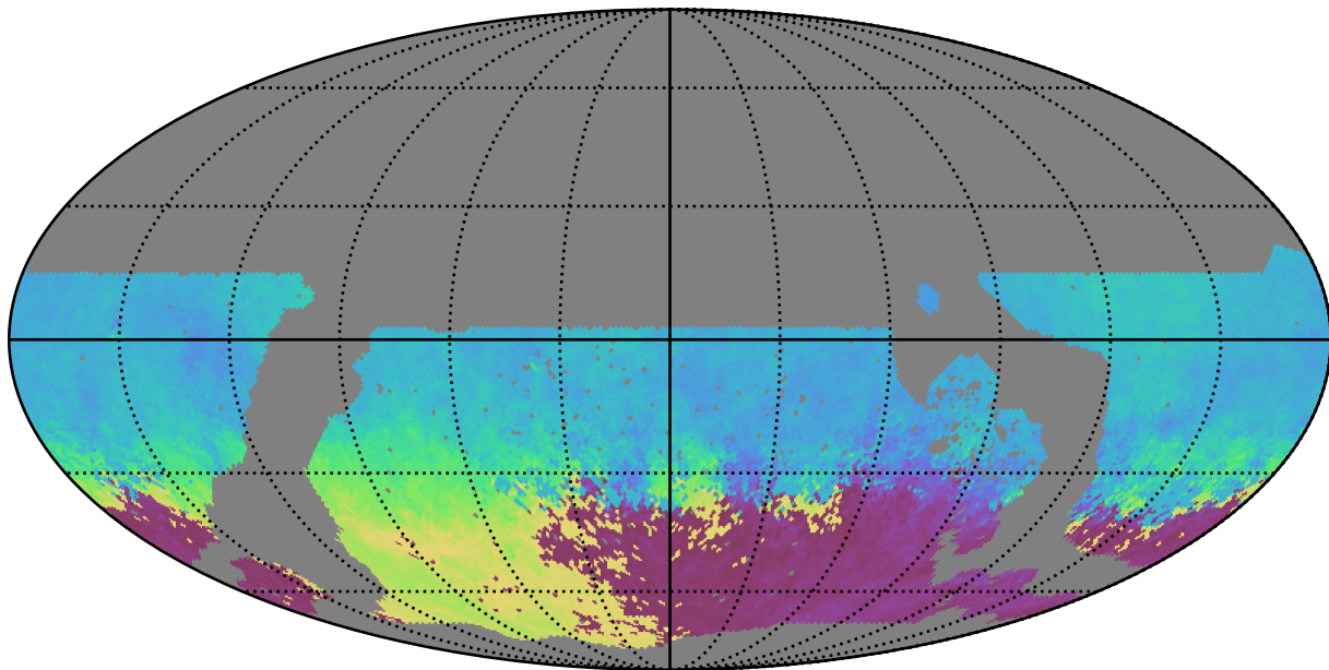
noroll_v3.4_10yrs WFD u band: AngleMean rotSkyPos
