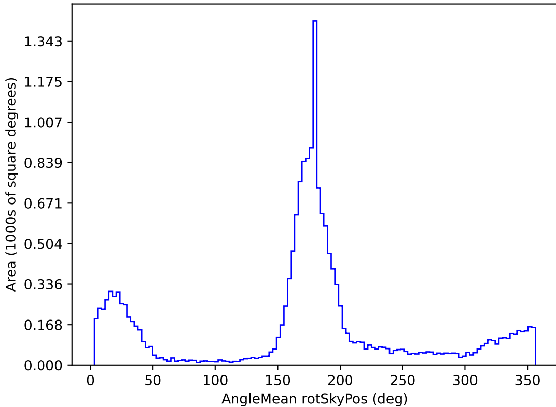
noroll_v3.4_10yrs WFD u band: AngleMean rotSkyPos
