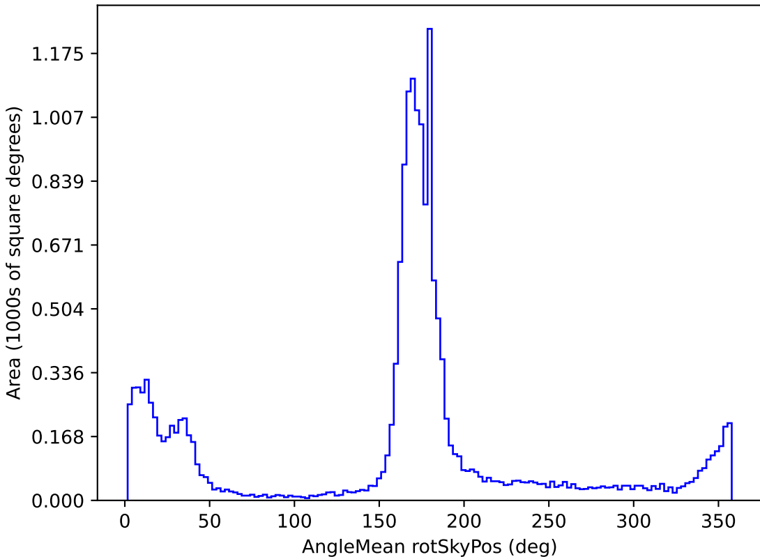
noroll_v3.4_10yrs WFD r band: AngleMean rotSkyPos
