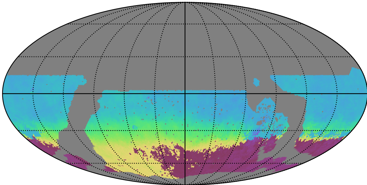
noroll_v3.4_10yrs WFD i band: AngleMean rotSkyPos
