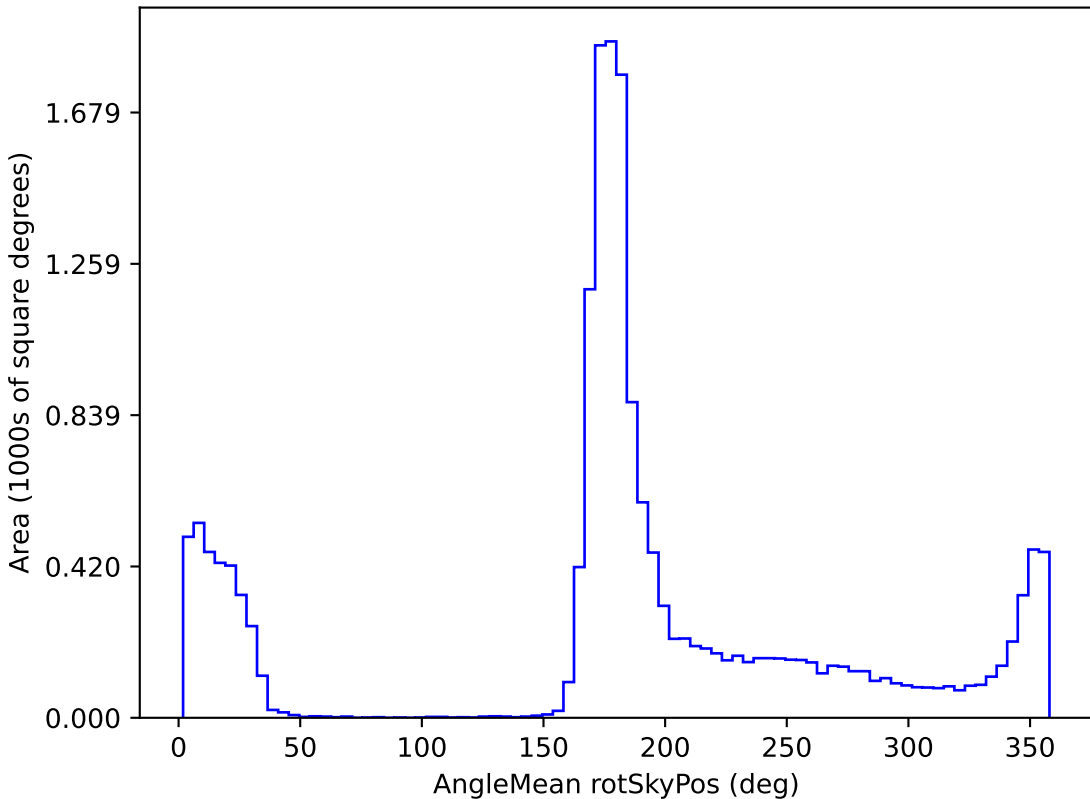
noroll_v3.4_10yrs WFD i band: AngleMean rotSkyPos
