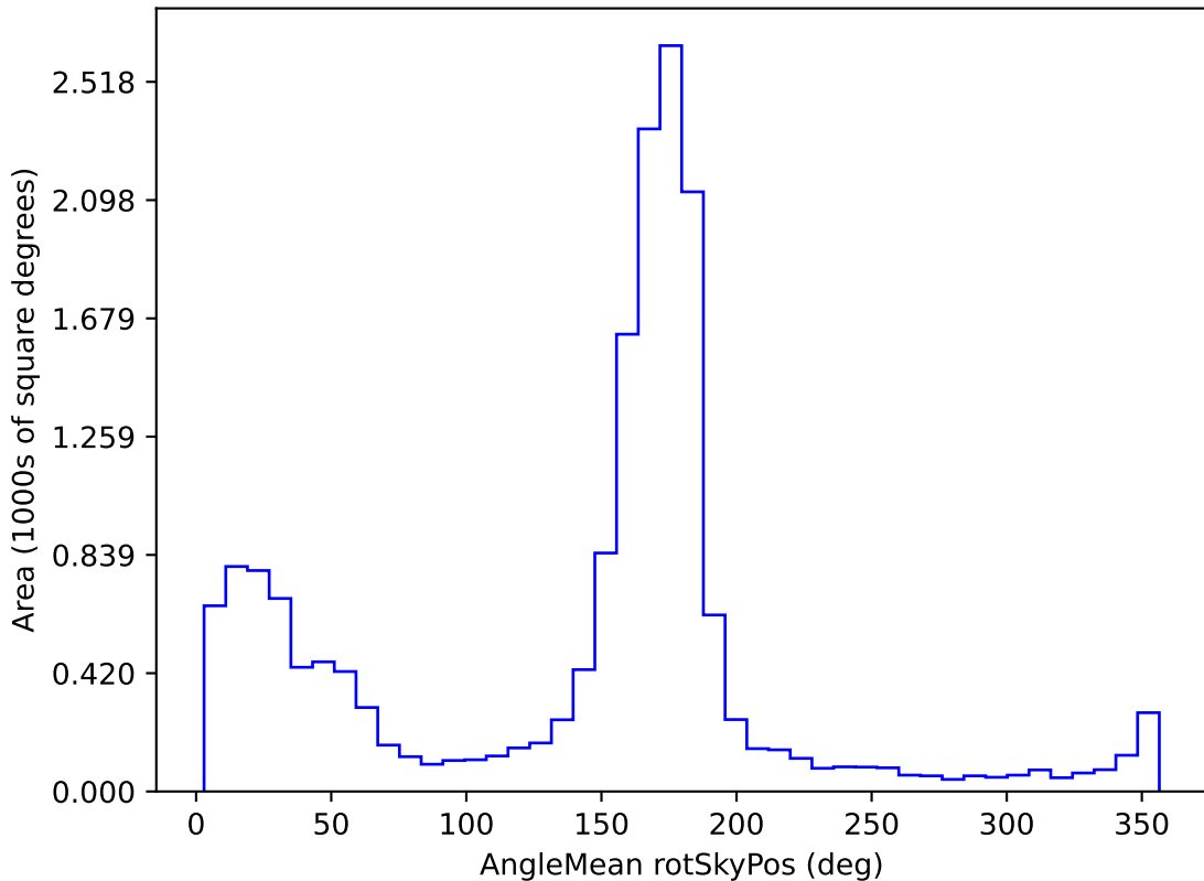
noroll_v3.4_10yrs WFD g band: AngleMean rotSkyPos
