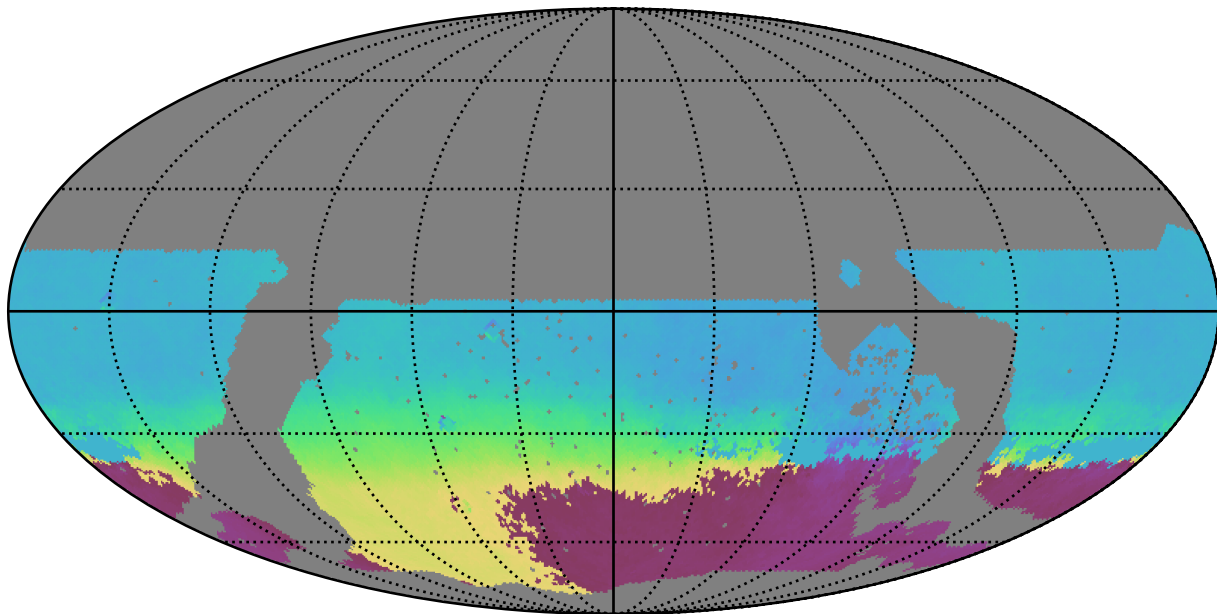
noroll_v3.4_10yrs WFD all bands: AngleMean rotSkyPos
